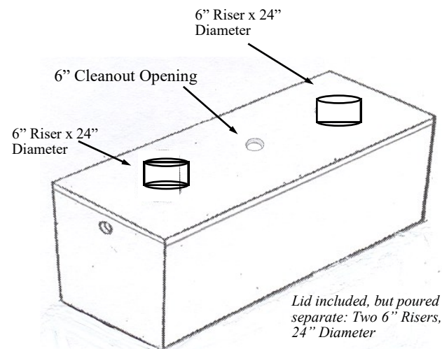
Septic Tank Lid designed with Two Risers, One Cleanout
